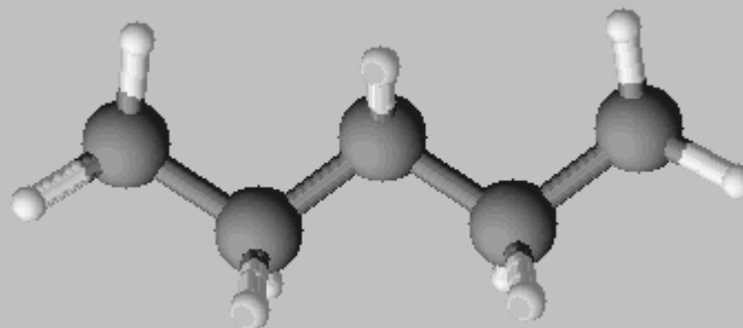
Pentane
